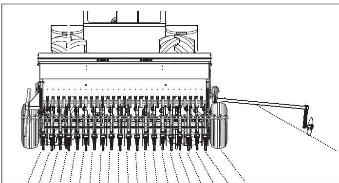
Figure 3S. Centre marking.
