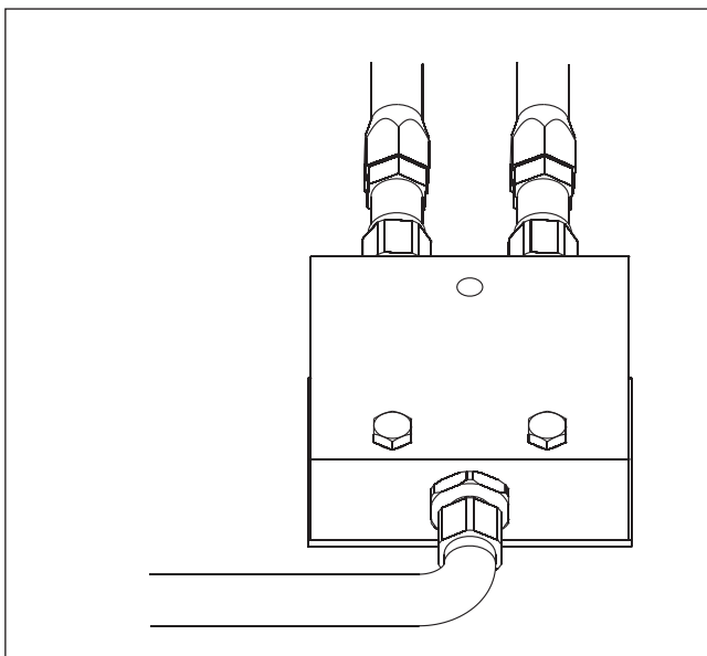
Figure 2C. The valve of the seed drill for the hydraulic marker
