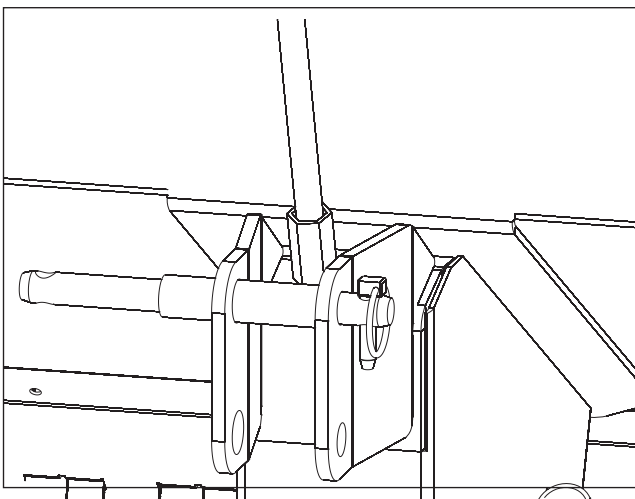
Figure 3N. Central coulters tightening.
