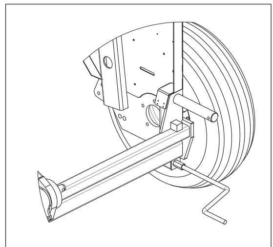
Figure 3P. Coulter tension, outer coulters.
