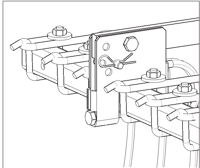
Figure 3U. Following harrow adjusted for heavy harrowing.
