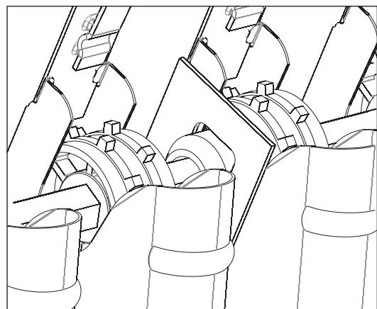
Figure 5B. Locking plates to sowing shaft.
